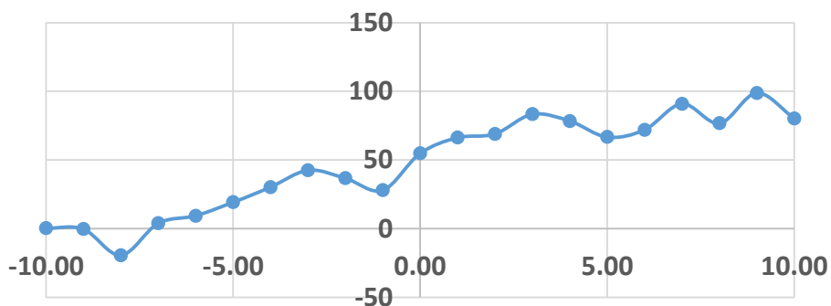
Forward Yaw ( \mu\text{rad} ) vs. Position (mm)
