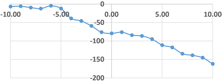
Backward Pitch (μrad) vs. Position (mm)
