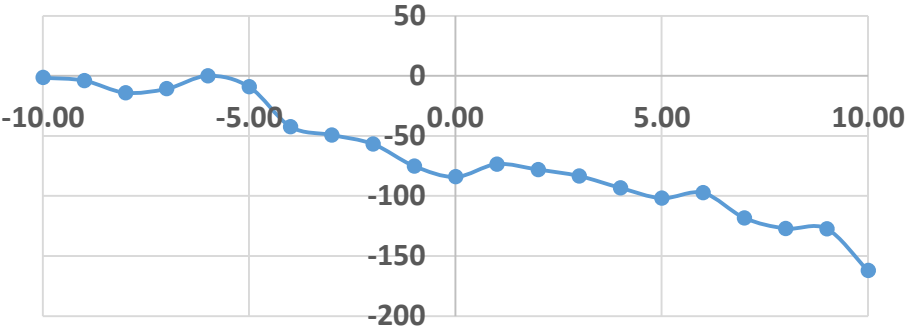
Forward Pitch (μrad) vs. Position (mm)
